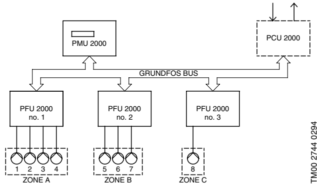
Example of Units Connected via GRUNDFOS BUS
