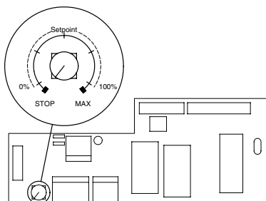
Function Selector in the PFU 2000
